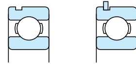
With snap ring groove With locating snap ring
